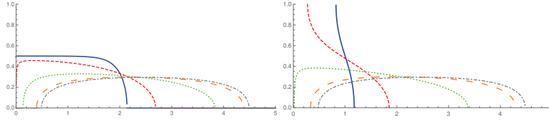
Рис. 1. Plots of the limit densities (14) (on the left) and (15) (on the right) for c = 4 and the values of \gamma : -10 (solid blue), -2 (dashed red), -0.5 (dotted green), -0.1 (sparsely dashed orange) -0.01 (dot-dashed gray).
