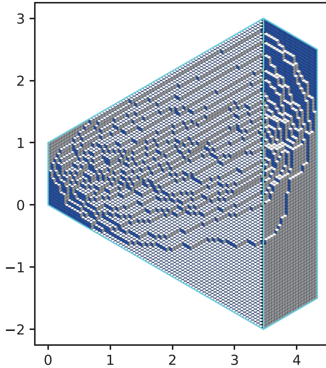
Рис. 4. Lozenge tiling of skew glued hexagon, Young diagrams \lambda, \bar{\lambda}' correspond to the positions of right (left) triangles on the main diagonal.
