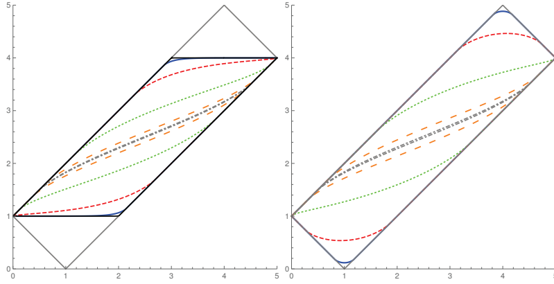
Рис. 2. Plots of the limit shapes for Young diagrams corresponding to the densities (14) (on the left) and (15) (on the right) for c = 4 and the values of \gamma (bottom to top): -10 (solid blue), -2 (dashed red), -0.5 (dotted green), -0.1 (sparsely dashed orange), -0.01 (dot-dashed gray), 0.01 (dot-dashed gray), 0.1 (sparsely dashed orange), 0.5 (dotted green), 2 (dashed red), 10 (solid blue). Solid black lines on the left panel correspond to \gamma = \pm\infty ( q = \text{const} ).
