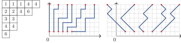
Рис. 3. A GL_6 -Young tableau, its row reading ( left ) and its column readings ( right ).
