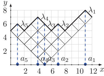
Diagram \lambda = (7, 4, 3, 3, 1) is rotated, thick black line is upper boundary f_n , row lengths \{\lambda_i\} correspond to the point positions \{a_i\} .
